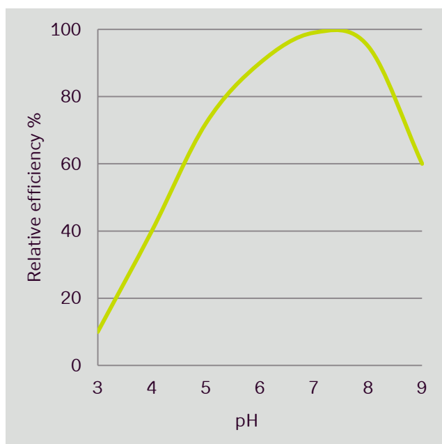
Fig. 1. pH profile of Novozymes Aquazym® 240 L
