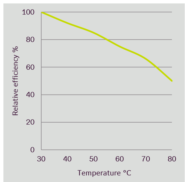
Fig. 2. Temperature profile of Novozymes Aquazym® 240 L
