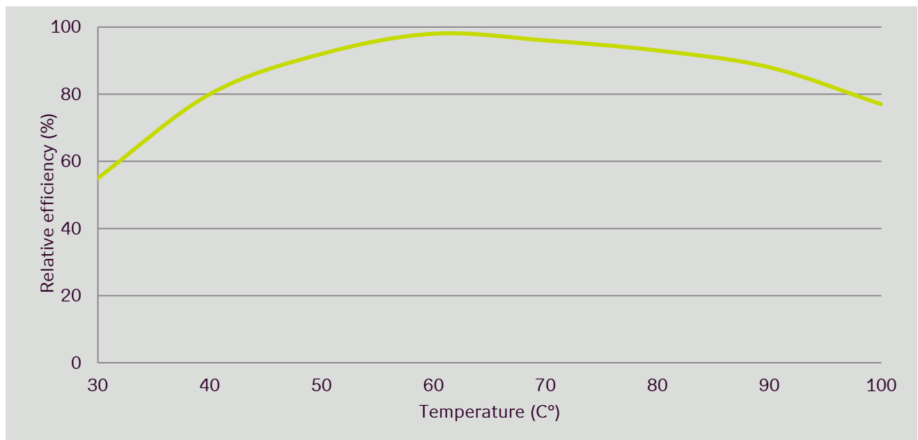
Fig. 2. Temperature profile of Novozymes Aquazym® Ultra 1200 N
